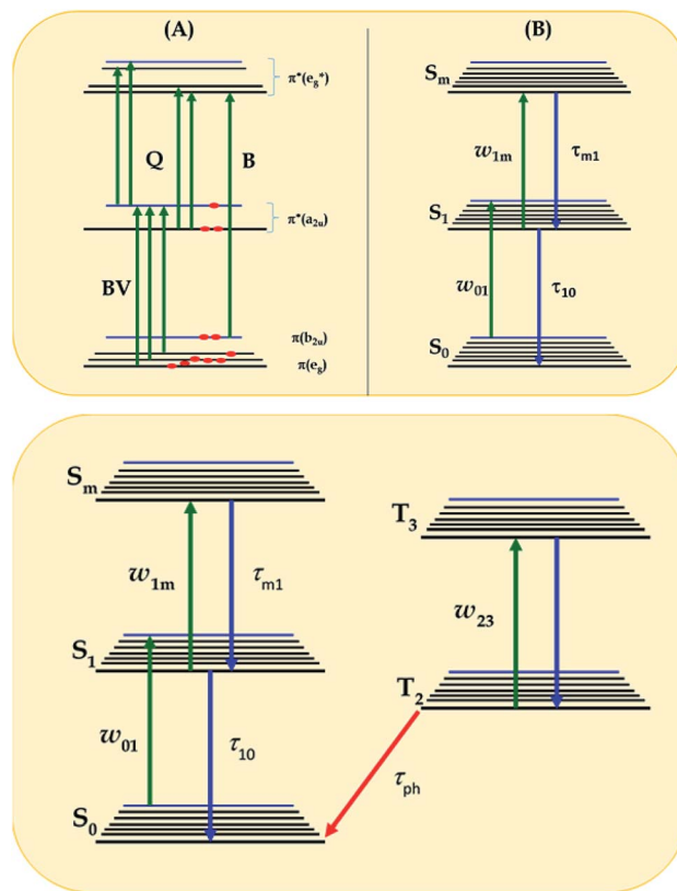
Fig. 5 (A) Diagram showing singlet excited states of \text{LnPc}_2 in comparison to that obtained by Orti et al. using Valence Effective Hamiltonian calculations; 44,53 (B) three-energy level diagram used to model the excited state cross-section spectrum within the rate equation model of eqn (1)–(3), according to ref. 56 and 57; and (C) general five-energy level diagram employed for the simulation of the NLO mechanisms of complexes 3a , 3b , 3a-TF and 3b-TF using eqn (6)–(12).
