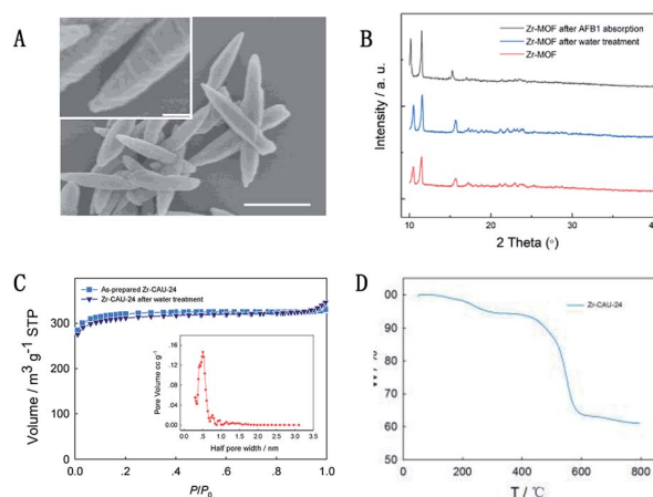
Fig. 2 Scanning electron microscopy images of prepared Zr-CAU-24 crystals with different magnification times. Scale bar: 1 \mu\text{m} (A), inset). PXRD of Zr-CAU-24 crystals before and after water treatment and AFB1 absorption, (B) and \text{N}_2 adsorption/desorption isotherms (C) of Zr-CAU-24 crystals before and after 24 h water treatment. TGA result of as-prepared Zr-CAU-24 crystals (D).
