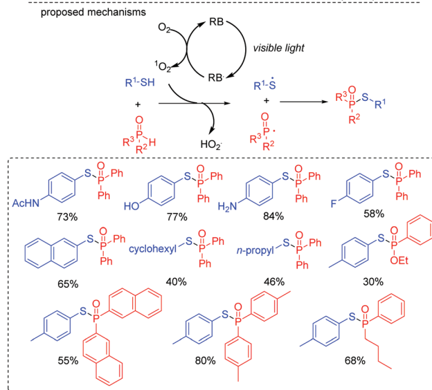
Scheme 24 Construction of S-P(O) bonds.
