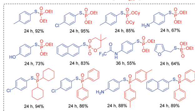
Scheme 25 Synthesis of thiophosphates.
