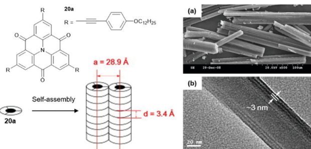
Fig. 21 Schematic representation of the two-step self-assembly of 20a into microrods. A representative SEM (a) and a TEM image (b) are also shown. 60 Figure reproduced with kind permission; © 2009 Elsevier B.V.
