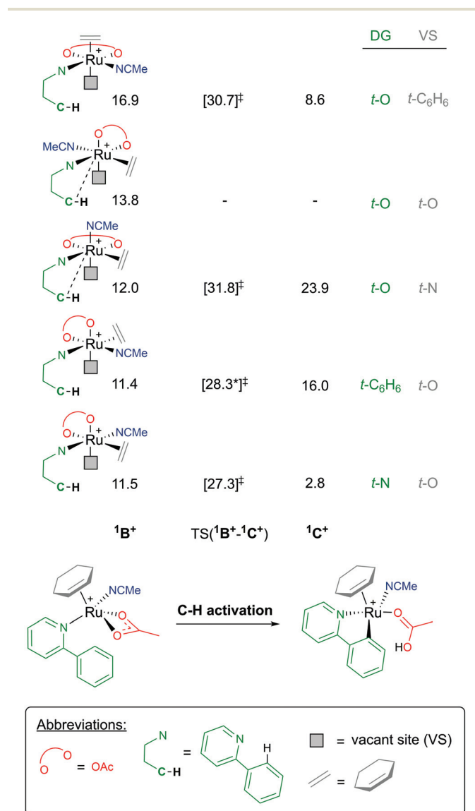
Fig. 8 BP86-D3BJ(BS2,MeCN)//BP86(BS1) free energy values at 120 °C for C–H activation of a-H for isomers of ^1\text{B}^+ , relative to A, [(\text{C}_6\text{H}_5)_2\text{Ru}(\text{OAc})_2] , in kcal mol -1 .
