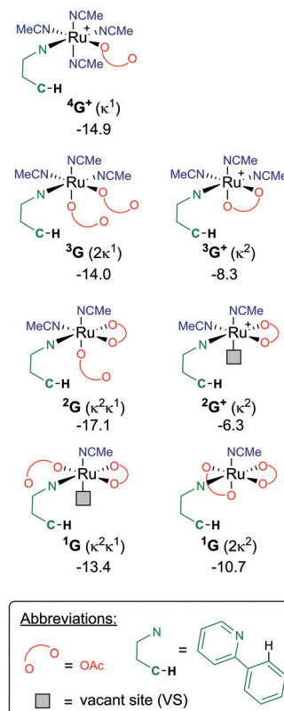
Fig. 9 BP86-D3BJ(BS2,MeCN)//BP86(BS1) free energy values at 120 °C for isomers of G, relative to A, [(\text{C}_6\text{H}_5)_2\text{Ru}(\text{OAc})_2] , in kcal mol -1 {chem-draws of each isomer do not necessarily represent the most stable intermediate energy quoted, but are to highlight the differences in each “G” species}.
