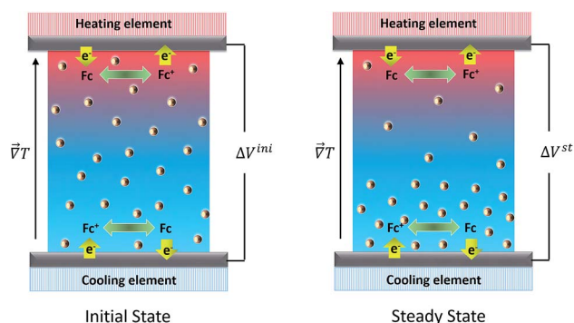
Fig. 1 Schematic images of an open-circuit thermocell containing redox molecules (e.g., \text{Fc}^+/\text{Fc} (ferrocenium)/ferrocene)) and charged nanoparticles. Left panel: Initial state immediately after the application of a temperature gradient where NP concentration is still homogeneous. Right panel: Steady state established after the completion of thermodiffusive movements of all charged species. Note that in the open-circuit configuration, there is no electric current flowing into and from the thermocell. Therefore both reduction and oxidation reactions occur at the hot and cold electrodes. In this example, the charged NPs move toward the cold region of the fluid, corresponding to a positive S_T . See the text for more explanation.
