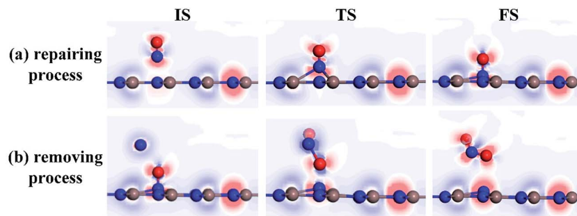
Fig. 7 ELF of different PM states. (a) Repairing process and (b) removing process. The red (blue) region represents charge accumulation (depletion).
