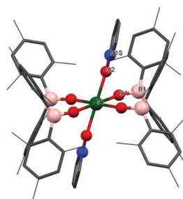
Fig. 3 Solid-state structure of 4 m . Hydrogen atoms are omitted and mesityl and pyridine oxide ligands are depicted as wireframe and capped sticks for clarity.
