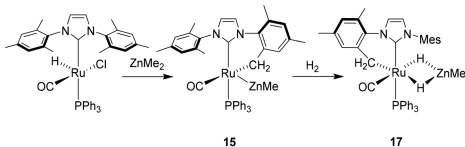
Scheme 6 Formation of [Ru( IMes )'(PPh_3)(CO)ZnMe] ( 15 ) and [Ru( IMes )'(PPh_3)(CO)(H)_2ZnMe] ( 17 ).
