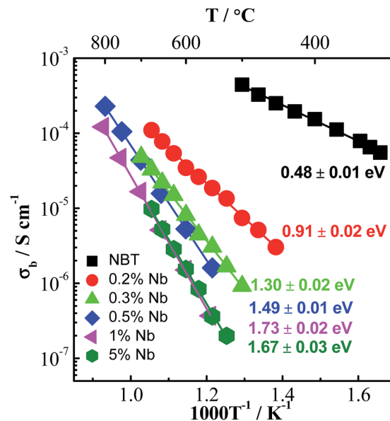
Fig. 8 Arrhenius plot of the bulk conductivity, \sigma_b , of Nb-doped NBT with a nominal composition Na 0.5 Bi 0.5 Ti 1-x Nb x O 3+0.5x . Activation energy for each composition is indicated in the figure. Replotted after ref. 29 and 34.
