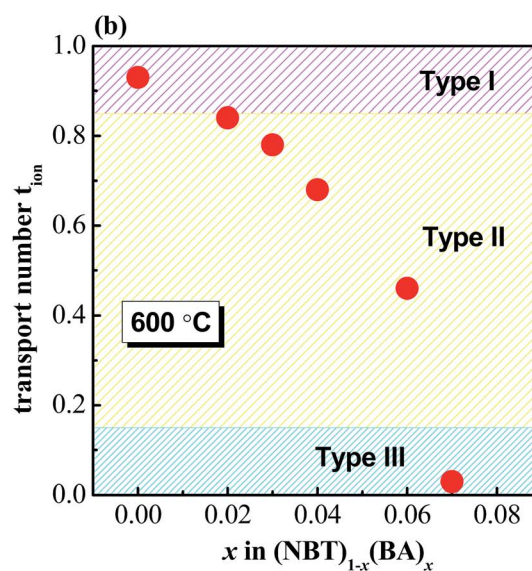
Fig. 7 (a) Arrhenius plots of the bulk conductivity and (b) oxide-ion transport number at 600 °C for the (NBT) 1-x (BiAlO 3 ) x ( 0 \leq x \leq 0.08 ) solid solutions. 48
