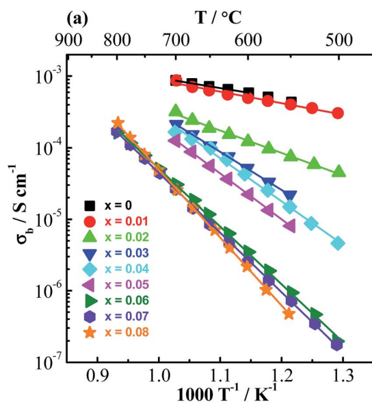
Fig. 7 (a) Arrhenius plots of the bulk conductivity and (b) oxide-ion transport number at 600 °C for the (NBT) 1-x (BiAlO 3 ) x ( 0 \leq x \leq 0.08 ) solid solutions. 48
