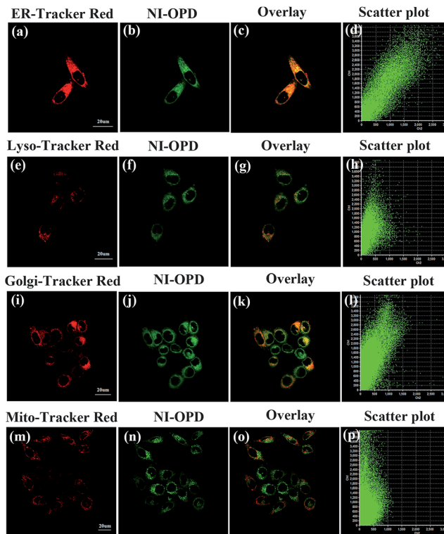
Fig. 4 The colocalization imaging of HeLa cells stained with NI-OPD ( 10 \mu\text{M} , \lambda_{\text{ex}} = 405 \text{ nm} , collected at 420\text{--}480 \text{ nm} ) with organelle dyes, including ER-Tracker Red ( 500 \text{ nM} , \lambda_{\text{ex}} = 559 \text{ nm} , collected at 590\text{--}640 \text{ nm} ), Lyso-Tracker Red ( 100 \text{ nM} , \lambda_{\text{ex}} = 559 \text{ nm} , collected at 580\text{--}610 \text{ nm} ), Golgi-Tracker Red ( 500 \text{ nM} , \lambda_{\text{ex}} = 559 \text{ nm} , collected at 590\text{--}640 \text{ nm} ), Mito-Tracker Red ( 100 \text{ nM} , \lambda_{\text{ex}} = 635 \text{ nm} , collected at 640\text{--}690 \text{ nm} ). Scale bar: 20 \mu\text{m} .
