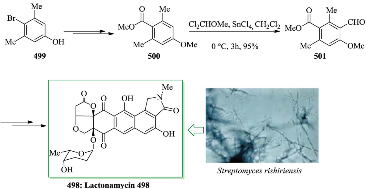
Scheme 107 Total synthesis of lactonamycin 498.
