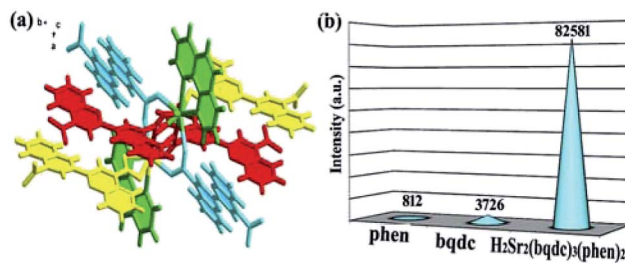
Fig. 2 (a) The crystal structure of the title complex. (b) The emission intensities of phen, bqdc and \text{H}_2\text{Sr}_2(\text{bqdc})_3(\text{phen})_2 .
