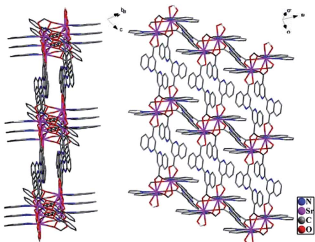
Fig. 1 Illustration of the \text{H}_2\text{Sr}_2(\text{bqdc})_3(\text{phen})_2 . All of the H atoms are omitted for clarity.
