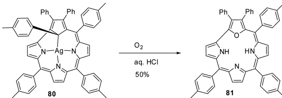
Scheme 20 Synthesis of 21-oxacorrole 81 from Ag(III) carbaacorrole 80 .
