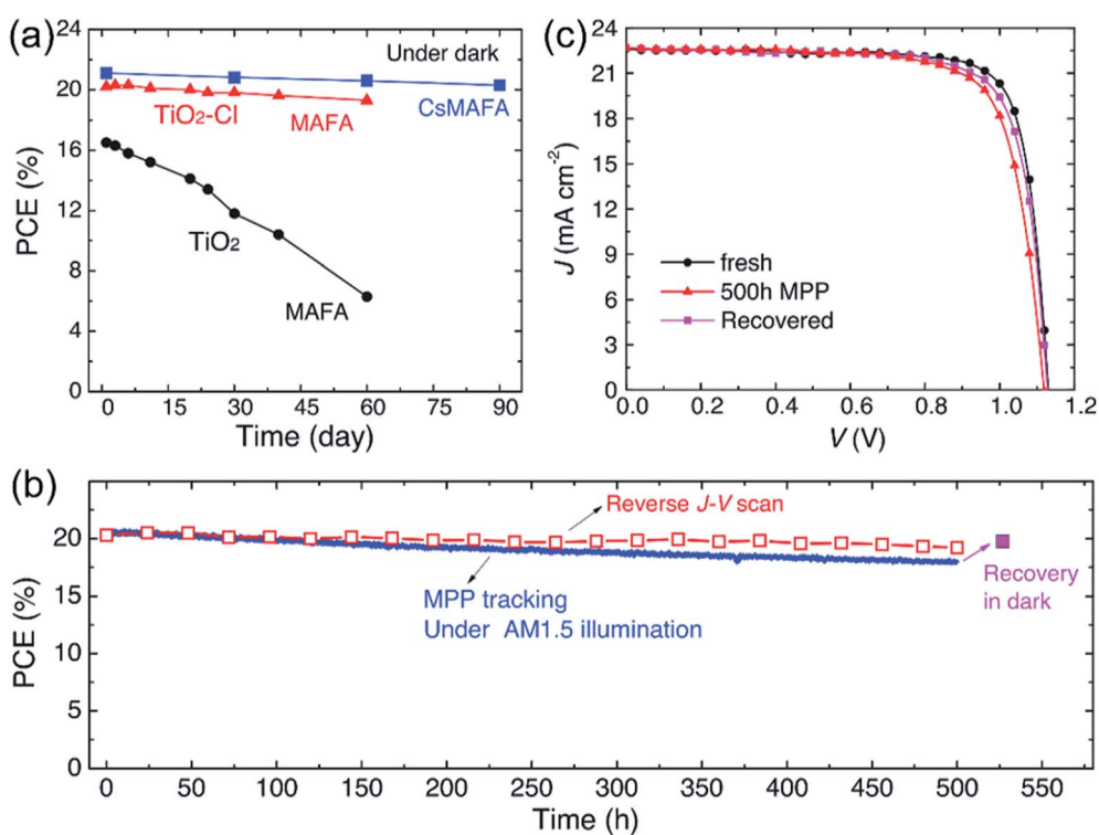
Fig. 25 Long-term device stability of PSCs with TiO 2 -Cl and TiO 2 . (a) Dark storage stability of non-encapsulated PSCs. (b) Continuous maximum power point tracking for 500 hours of a high performance unsealed CsMAFA cell with TiO 2 -Cl in nitrogen atmosphere under constant simulated solar illumination. (c) J - V curves of the PSCs (CsMAFA) from (b) at various stages. 31
