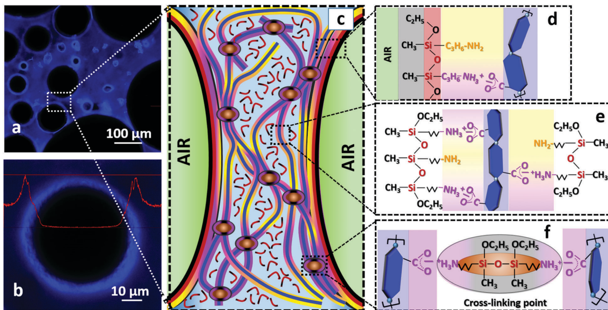
Fig. 6 Stability mechanisms of the TCNF/AS foams. (a) Fluorescent optical microscopy images of TCNF/AS 3_wf (10.8) with (b) magnification of a single air bubble. The TCNFs are dyed with a blue fluorescent colorant. The red line on (b) represents the emission spectral profile. (c) Schematic illustration of the structure of the foam lamella after 12 h of drying: the green half spheres represent part of the air bubbles, the light blue background is the water medium, the blue continuous lines sketch the TCNFs and the red lines with black ends sketch short organosilica polymers. Molecular representation of (d) assembly of TCNF/AS at the air/water interface, (e) AS coated-TCNFs and (f) TCNFs and AS crosslinking points. The yellow color represents non-protonated amine groups of AS, pink – attractive electrostatic and van der Waals interactions, black – unreacted ethyl groups and methyl groups, red – siloxane bonds between neighbor AS molecules and in organosilica chains. The blue hexagons connected with light blue balls represent sugar rings with glycosidic bonds in a single cellulose chain as a simplified representation of TCNFs. Only a few deprotonated carboxylic groups are shown for simplicity.
