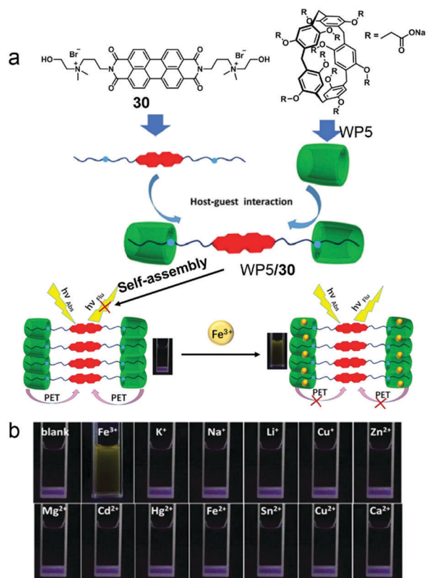
Fig. 23 (a) Chemical structures of the host and guest compounds and a cartoon representation of the Fe^{3+} ion sensing mechanism. (b) Photographs of WP5/30 supra-amphiphile solutions after adding various metal ions under UV light. Adapted with permission from ref. 95. Copyright 2017 American Chemical Society.
