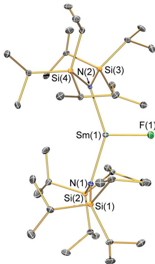
Fig. 1 Molecular structure of [\text{Sm}(\text{N}^{\dagger\dagger})_2(\text{F})] (2-F) with selective atom labelling. Displacement ellipsoids set at a 30% probability level and hydrogen atoms are omitted for clarity. Selected bond lengths [Å]: Sm(1)–F(1) 2.051(3), Sm(1)–N(1) 2.353(3), and Sm(1)–N(2) 2.334(3). Selected bond angles [°]: N(1)–Sm(1)–N(2) 143.29(12), N(1)–Sm(1)–F(1) 106.81(12), and N(2)–Sm(1)–F(1) 108.63(12).
