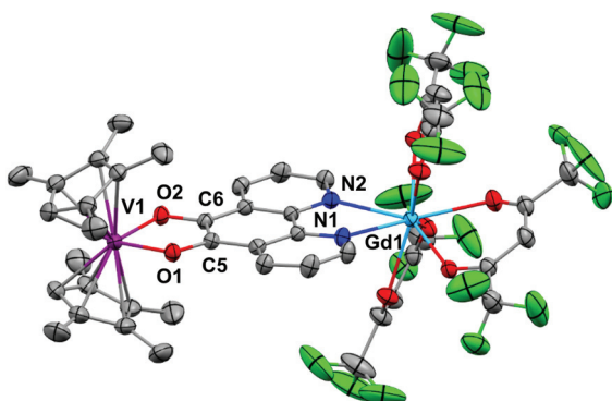
Fig. 6 Molecular structure of 6 . Hydrogen atoms and solvent of crystallisation omitted for clarity. Thermal ellipsoids drawn at 50% probability. Selected distances ( \text{\AA} ) for 5 : \text{Y1-N1} 2.48(1), \text{Y1-N2} 2.49(1), \text{C5-C6} 1.38(2), \text{C6-O2} 1.35(1), \text{C5-O1} 1.34(2), \text{V1-O1} 1.975(8), \text{V1-O2} 1.977(9) and 6 : \text{Gd1-N1} 2.532(2), \text{Gd1-N2} 2.527(2), \text{C5-C6} 1.387(3), \text{C6-O2} 1.333(3), \text{C5-O1} 1.333(3), \text{V1-O1} 1.9869(18), \text{V1-O2} 1.9862(18).
