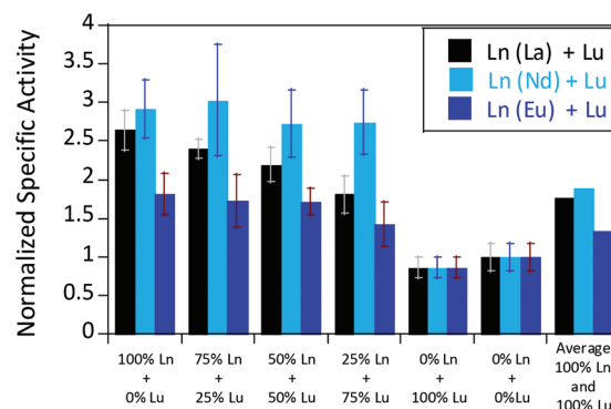
Fig. 6 Mixed Ln normalized specific activities ( n = 3 ) of 200 nM Eu-MDH in the presence of 20 \mu\text{M} \text{LnCl}_3 ( \text{Ln} = \text{Lu} + \text{La}/\text{Nd}/\text{Eu} ). Conditions: 20 mM PIPES pH 7.2, 1 mM PES, 1 mM KCN, 100 \mu\text{M} DCPIP, 50 mM MeOH, 45 °C.
