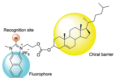
Fig. 1 Design strategy of NI-cholesterol 1 .
