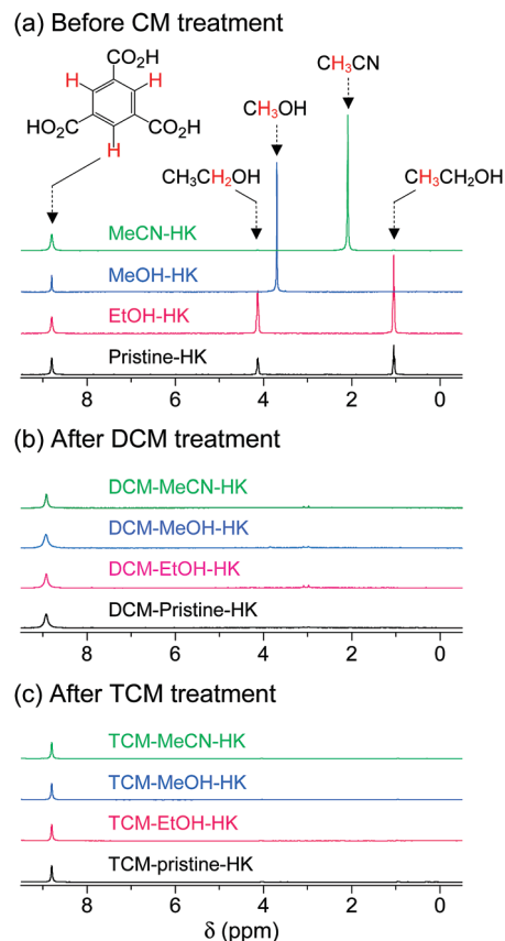
Fig. 4 ^1\text{H} NMR spectra of pristine-, EtOH-, MeOH-, and MeCN-coordinated HKUST-1 (a) before chloromethane treatment, (b) after DCM treatment, and (c) after TCM treatment. NMR spectra were measured after completely dissolving the powder samples in \text{D}_2\text{SO}_4 . Reprinted (adapted) with permission from ref. 68 and 70. Copyright (2015 and 2018) American Chemical Society.
