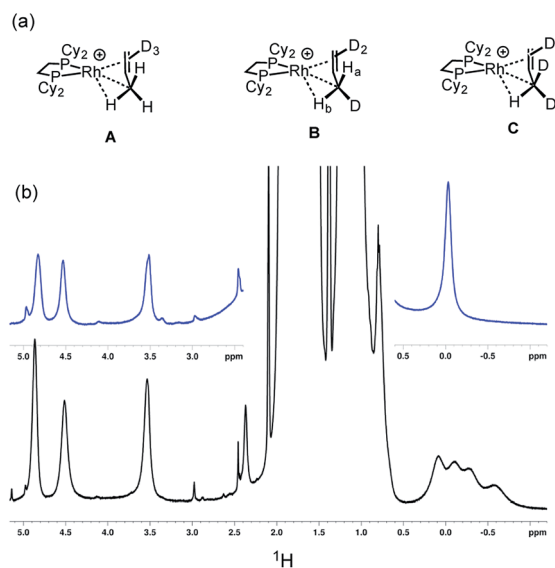
Scheme 9 (a) Isotopomers [\mathbf{1}\text{-}(\text{d}_3\text{-propene})][\text{BAR}^{\text{F}}_4] highlighting the methyl substitution patterns. (b) ^1\text{H} NMR spectra (193 K, \text{CD}_2\text{Cl}_2 ) of a sample prepared by the solid/gas route after 16 hours. Top, [\mathbf{1}\text{-}(\text{propene})][\text{BAR}^{\text{F}}_4] ; bottom, [\mathbf{1}\text{-}(\text{d}_3\text{-propene})][\text{BAR}^{\text{F}}_4] .
