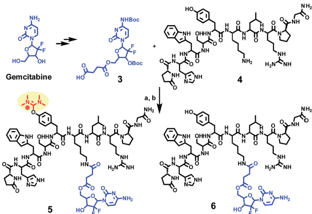
Scheme 1 Synthesis of a gemcitabine-GnRH conjugate 6 and its uronium side product 5. (a) HATU (1.5 eq.), DIPEA (5 eq.), DMF; (b) TFA/TIS/H 2 O (95/2.5/2.5%).
