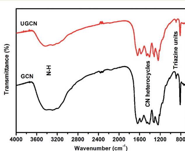
Fig. 2 FTIR spectra for as-prepared GCN and UGCN samples.
