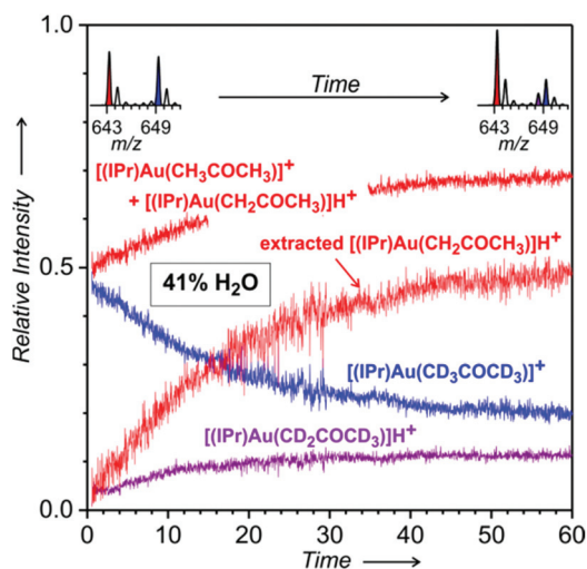
Fig. 5 Time evolution of the relative intensities of the signals at m/z 643 [(IPr)Au(CH 3 COCH 3 ) + + [(IPr)Au(CH 2 COCH 3 )H + in red), m/z 648 [(IPr)Au(CD 2 COCD 3 )H + in violet), and m/z 649 [(IPr)Au(CD 3 COCD 3 ) + in blue – this intensity was corrected for the 13 C contribution of the signal at m/z 648). Under the assumption that the complexes with intact acetone molecules are formed in the 1 : 1 ratio during the whole experiment, the evolution of the signal intensity of [(IPr)Au(CH 2 COCH 3 )H + was extracted as a difference between the intensities of m/z 643 and m/z 649. Experiment: [(IPr)AuBF 4 ] (358 μg) was dissolved in dioxane (0.2 ml) and H 2 O (0.14 ml – 41% v/v) and left to react for 15 hours. Then, a 1 : 1 mixture of CH 3 COCH 3 and CD 3 COCD 3 (1.4 ml) was added and the solution was immediately monitored by ESI-MS.
