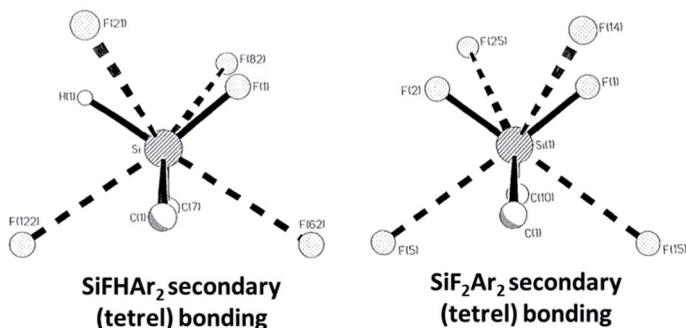
Fig. 11 Crystal structure of SiFHA r 2, Ar = C 6 H 2 (CF 3 ) 3 (top), with secondary (tetrel) bonding shown as dashed bonds and primary bonding (solid lines) and secondary bonding (dashed lines) at Si in SiFHA r 2 and SiF 2 Ar 2 (bottom). Secondary (tetrel) Si···F bonds are longer than primary (covalent) Si–F bonds. Secondary bonds trans to F are shorter than those trans to C. Adapted from ref. 57 with permission from Elsevier.
