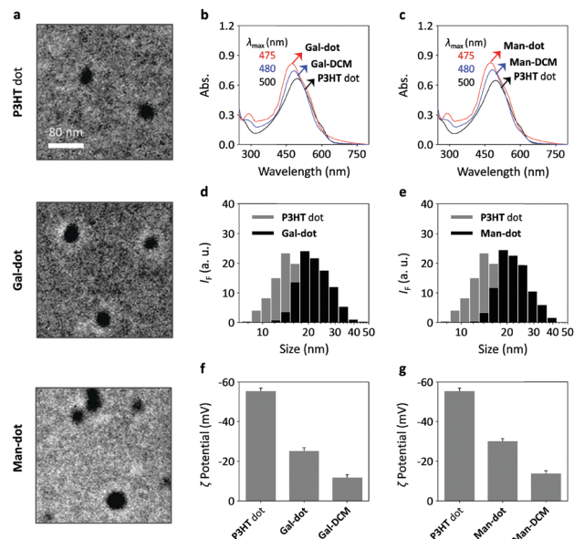
Fig. 2 (a) Transmission electron microscopy images of P3HT nanodot (100 ppm), Gal-dot (16 \mu M/100 ppm) and Man-dot (16 \mu M/100 ppm). Stacked UV-vis absorbance spectra of (b) Gal-dot (50 \mu M), P3HT nanodot (20 ppm) and Gal-dot ( Gal-DCM / P3HT nanodots = 50 \mu M/20 ppm) and (c) Man-dot (50 \mu M), P3HT nanodots (20 ppm) and Man-dot ( Man-DCM / P3HT nanodot = 50 \mu M/20 ppm) measured in Tris-HCl buffer (0.01 M, pH 7.4). Dynamic light scattering analysis of (d) P3HT nanodots (16 ppm) and Gal-dot ( Gal-DCM / P3HT nanodots = 1 \mu M/16 ppm) and (e) P3HT nanodots (16 ppm) and Man-dot ( Man-DCM / P3HT nanodots = 1 \mu M/16 ppm) measured in Tris-HCl buffer (0.01 M, pH 7.4). Zeta potential of (f) Gal-DCM (1 \mu M), P3HT nanodots (16 ppm) and Gal-dot ( Gal-DCM / P3HT nanodots = 1 \mu M/16 ppm) and (g) Man-DCM (1 \mu M), P3HT nanodots (16 ppm) and Man-dot ( Man-DCM / P3HT nanodots = 1 \mu M/16 ppm) measured in deionized water.
