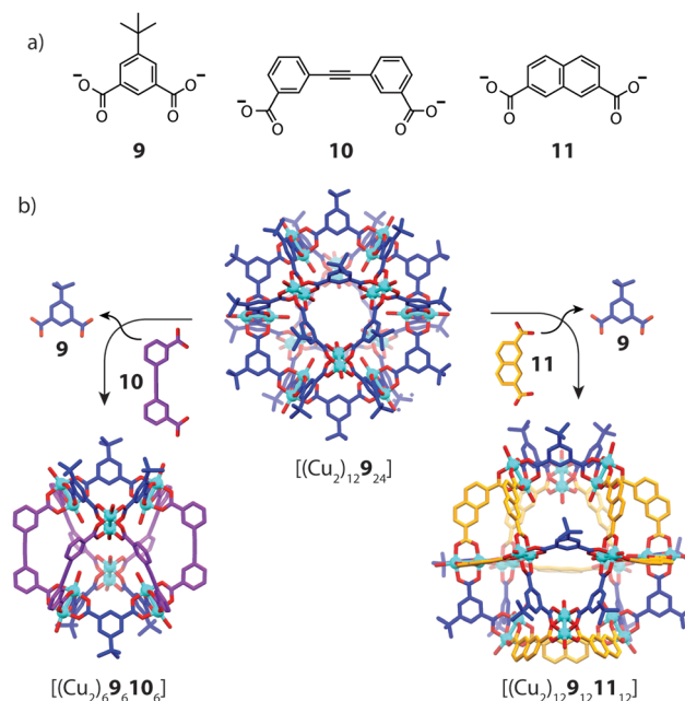
Fig. 7 (a) Bent dicarboxylate ligands 9–11 bearing angles of 120^\circ , 60^\circ and 120^\circ respectively; (b) transformation of the homoleptic [(Cu_2)_{12} 9_{24}] cage to heteroleptic species [(Cu_2)_6 9_6 10_6] (left) and [(Cu_2)_{12} 9_{12} 11_{12}] (right) by ligand substitution.
