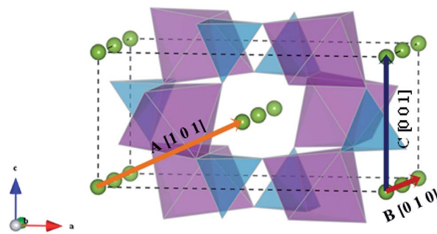
Fig. 3 Schematic representation of the possible migration paths in olivine-type \text{AFeyPO}_4 ( A = \text{Li}^+ or \text{Na}^+ ). Blue: \text{PO}_4 tetrahedra; purple: \text{FeO}_6 octahedra; green: Li/Na.
