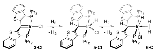
Scheme 4 Addition of H 2 to 3·Cl .
