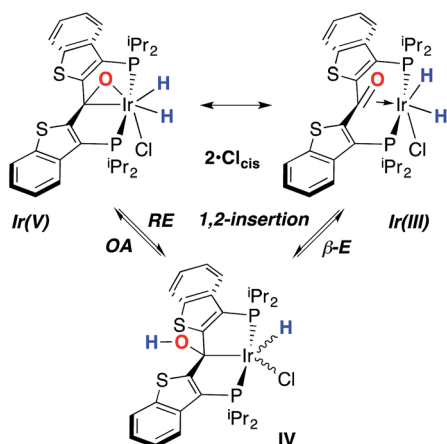
Scheme 5 Two views of the conversion of 2 \cdot \text{Cl}_{cis} to IV .
