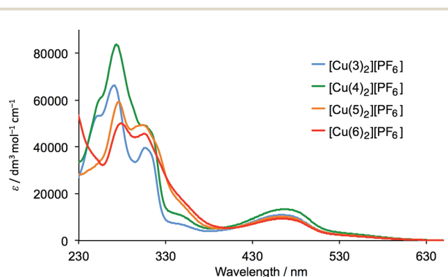
Fig. 2 Solution ( CH_2Cl_2 ) absorption spectra of complexes [Cu(L_{ancillary})_2][PF_6] with L_{ancillary} = 3-6 ( 5 \times 10^{-5} \text{ mol dm}^{-3} ).
