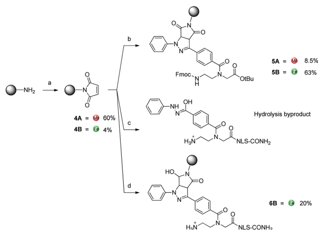
Fig. 5 Photoclick reaction. (a) Maleic anhydride, AcOH, 8 h, reflux. (b) 9 , ACN, 302 nm, 1 h, RT. (c) NLS-tetra, DMSO or ACN : PBS (5 : 1), 302 nm, 30 min, RT. (d) NLS-tetra, DMSO, 302 nm, 1 h, RT. All amine groups in the peptide sequence are present as TFA salts.
