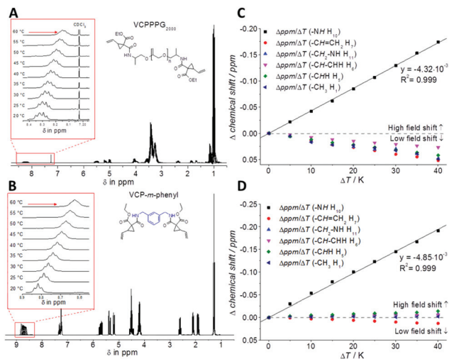
Fig. 2 (A + B) Variable-temperature ^1\text{H-NMR} experiments of VCP-PPG _{2000} and VCP- m -phenyl (0.5 mM in \text{CDCl}_3 ) between 20–60 °C. (C + D) Graphical plot of chemical shift within ^1\text{H-NMR} experiments. With increased temperature a decreased deshielding effect is anticipated, as a partial rupture of the H-bonds occurs.
