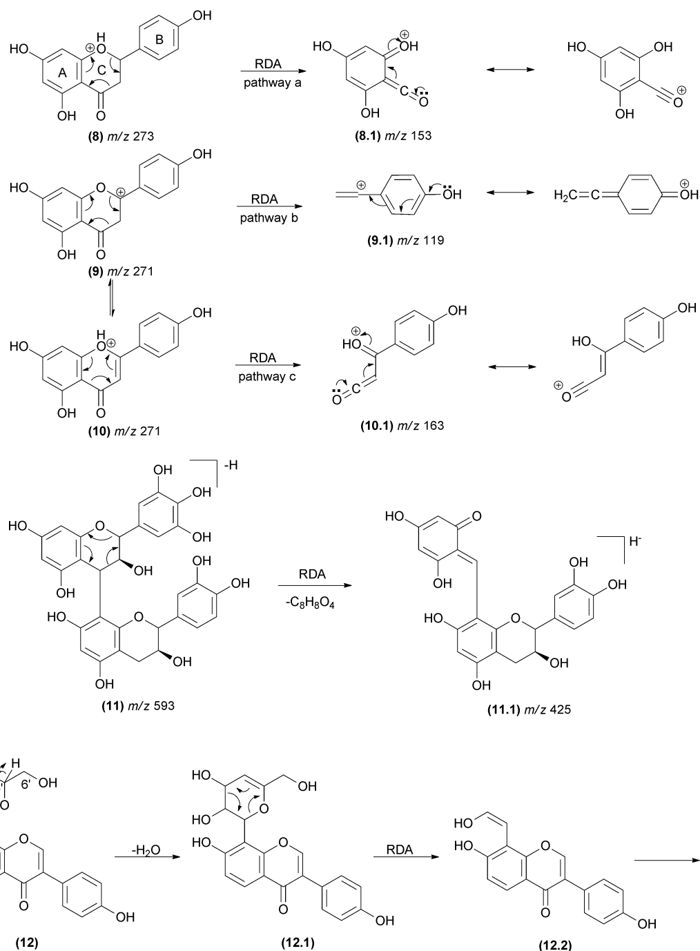
Fig. 9 RDA mechanisms involving the C-ring of flavonoids (8–10) and proanthocyanidins (10) and sugar units in natural products (12). The double bond present in the C-ring of flavones, flavonols, chalcones and isoflavones leads to an additional pathway (pathway c).
