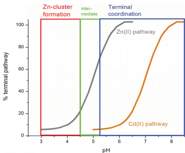
Fig. 9 Change in Zn(II) metalation pathway as a function of pH (grey line) compared to Cd (orange line). Demetalation begins to occur at \text{pH} < 4.5 so the curve was extrapolated to \text{pH} 3 based on the Cd metalation data. At the lowest physiologically relevant pH around 5.5 the binding pathway is greater than 80% terminal (blue box) and only forms clusters below \text{pH} 4.5 (red box).
