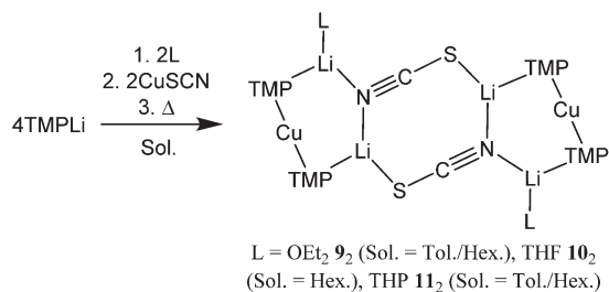
Scheme 3 Synthesis of 9–11 .
