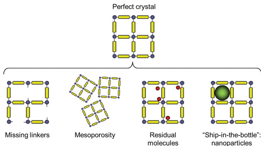
Fig. 1 Possible scenarios of structural deviation from the ideal crystal considered in this study. From left to right: missing linkers, the presence of mesopores, guest molecules such as the residual solvent and purposefully introduced nanoparticles.
