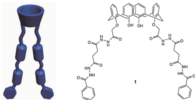
Scheme 1 Structure of gelator 1 and schematic representation.
