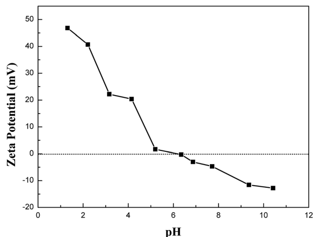
Fig. 7 Zeta potential of CMB at different solution pH.
