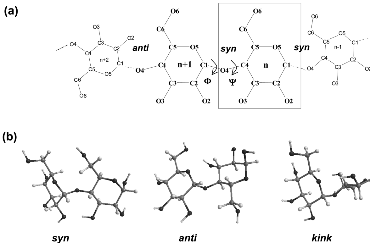
Fig. 1 (a) Schematic representation for a cyclodextrin showing the atomic numbering. Each individual glucose unit is designated by a number "n". Atoms are identified by a letter and a number that indicates its position in the glucose. (b) Relative conformations of neighbor glucoses: syn , anti and kink .
