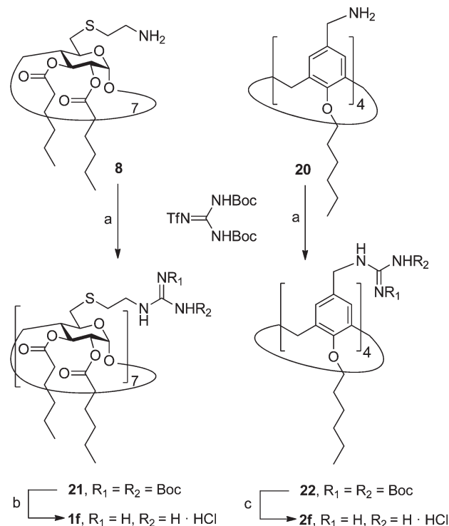
Scheme 4 Synthesis of polyguanidino \beta CD and CA_4 derivatives 1f and 2f . Reagents and conditions: (a) TfN=NHTf , DCM, rt, 12 h, 99% (for 21 ) or 48 h, 91% (for 22 ); (b) (i) 1 : 1 TFA-DCM, rt, 3 h; (ii) 0.1 M HCl, 99%; (c) TES, dioxane, 0.1 M HCl, rt, 24 h, quantitative.
