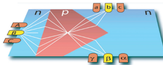
Fig. 89 Prism-shaped focusing beam-splitter in a ballistic graphene n-p-n junction. Electrons emitted from contact B are distributed between contacts \beta and \gamma . Adapted from ref. 143.
