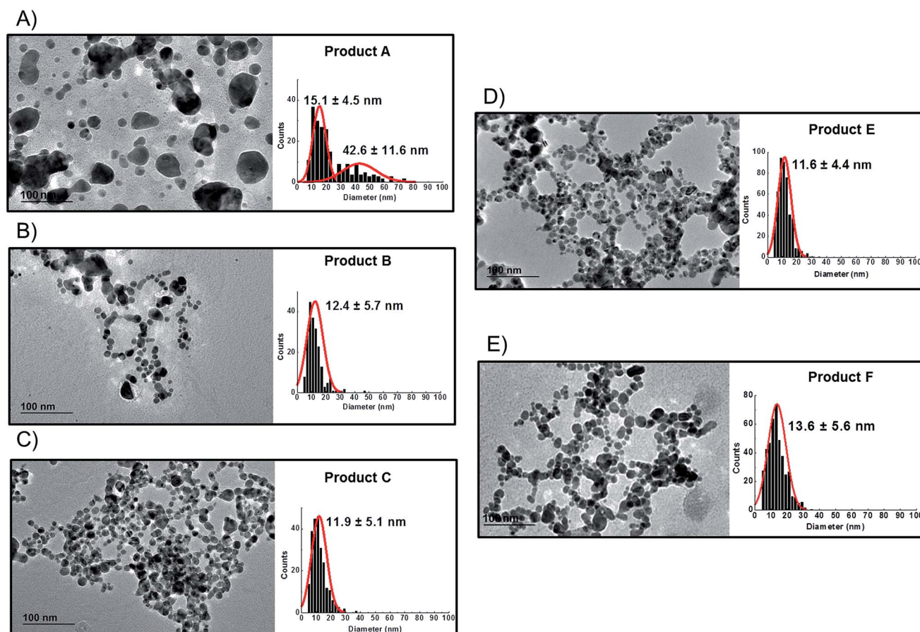
Fig. 3 TEM images and particle size distributions of consumer products; (A): Product A; (B): Product B; (C): Product C; (D): Product E; (E): Product F. Product D did not show any presence of detectable silver nanoparticles on TEM analysis.
