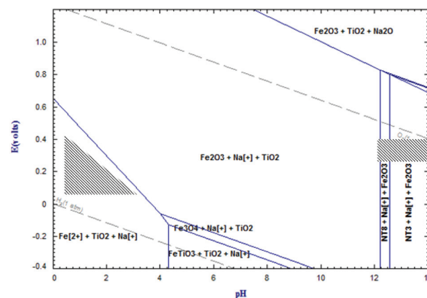
Fig. 16 The E_h -pH diagram of the system Na-Ti-Fe-O calculated by Fact-Sage 6.4 software at 70^\circ C . NT3: Na_2TiO_3 , NT8: Na_8Ti_5O_{14} . 66
