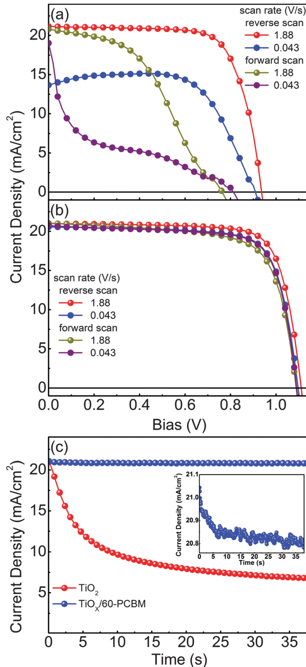
Fig. 2 J - V curves for photovoltaic devices FTO/ \text{TiO}_2 / \text{CH}_3\text{NH}_3\text{PbI}_3 /spiro-MeOTAD/Au (a) and FTO/ \text{TiO}_x/60\text{-PCBM}/\text{CH}_3\text{NH}_3\text{PbI}_3 /spiro-MeOTAD/Au (b) measured with different scan rates ( \text{V s}^{-1} ) and different scan directions under AM 1.5G white light illumination with an intensity of approximately 100 \text{ mW cm}^{-2} . Note that the devices were exposed for 10 s to white light before testing. No pre-polarization has been performed. (c) Corresponding short-circuit current density transients during illumination.
