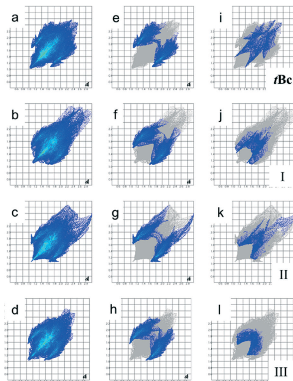
Fig. 4 Fingerprint plots for I_B , I_P , II_P and III_P . The left-hand column shows the complete fingerprint plots, the middle column shows only the C-H\cdots\pi interactions and the column on the right shows both the O\cdots H(O) and O\cdots H(C) interactions.
