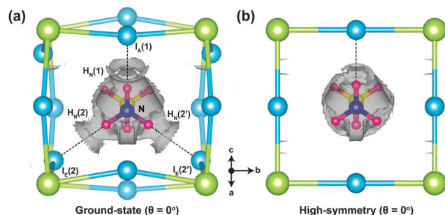
Fig. 4 Non-covalent interaction density isosurfaces for (a) the ground-state ( \theta = 0^\circ ) and (b) high-symmetry structures ( \theta = 0^\circ ). The reduced gradient density cut-off is 1.0 au.
