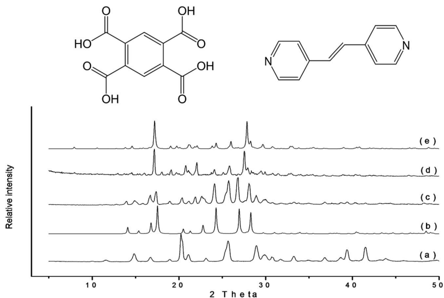
Fig. 15 Demonstration of the enhanced kinetics of cococrystal formation upon addition of a few drops of methanol to the grinding jar. PXRD patterns for (a) tetracarboxylic acid, (b) bipyrindyl, (c) outcome of neat grinding for 60 minutes (as the sum of the reactants), (d) the product obtained when a few drops of methanol are added and (e) the simulated pattern for the cococrystal.
