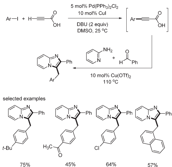
Scheme 63 Four-component reaction for the synthesis of imidazo[1,2-a]pyridines.
